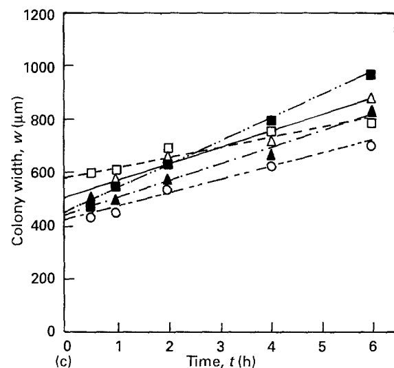
Figure 3 Variation of the maximum width of the DP colony ( w ) as a function of time ( t ) in: (a) uncoated; (b) Ag-coated; and (c) Cu-coated specimens. Load P = 1 kg ( \circ ), 5 kg ( \triangle ), 10 kg ( \square ), 20 kg ( \blacktriangle ) and 40 kg ( \blacksquare ).
